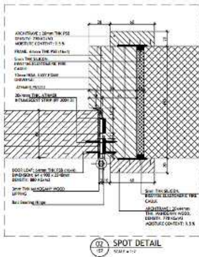
Figure 7: Spot Detail 2
