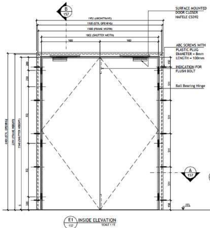
Figure 3: Inside Elevation
