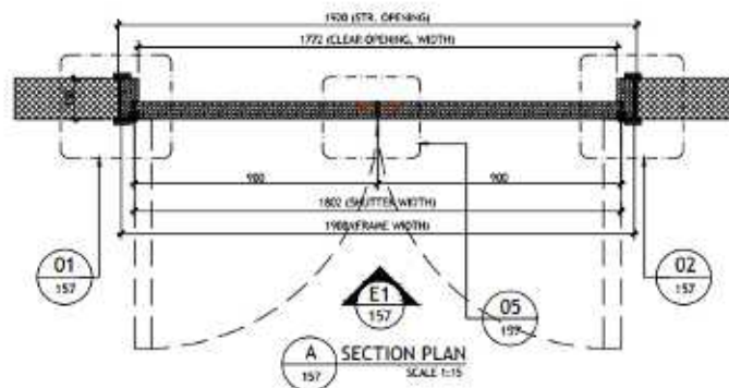
Figure 4: Section Plan
