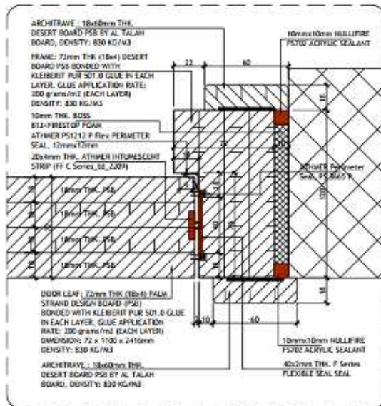
02 SPOT DETAIL SCALE = 1:2
