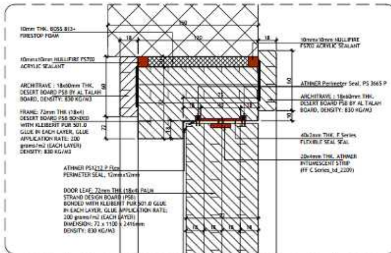
03 SPOT DETAIL SCALE = 1:1
