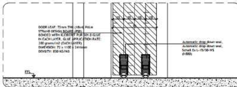
04 SPOT DETAIL SCALE = 1:1
