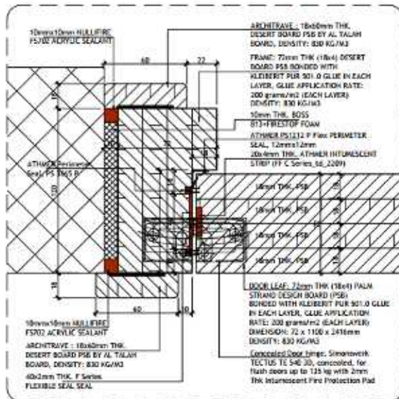
01 SPOT DETAIL SCALE = 1:2
