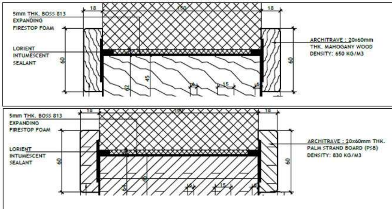
Figure 4. Architrave and frame cross section of door 1 and 2 respectively.
