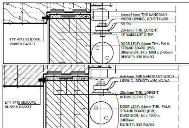
Figure 3. Top edge cross-section of door 1 and door 2 respectively.
