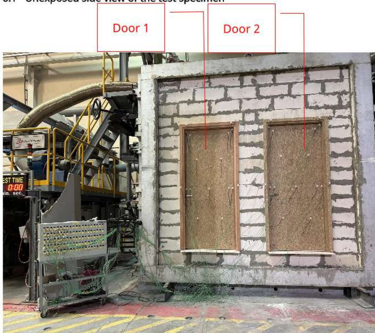
Photo 1. At 00:00 seconds into the test.
