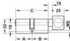
Thumbturn cylinder
