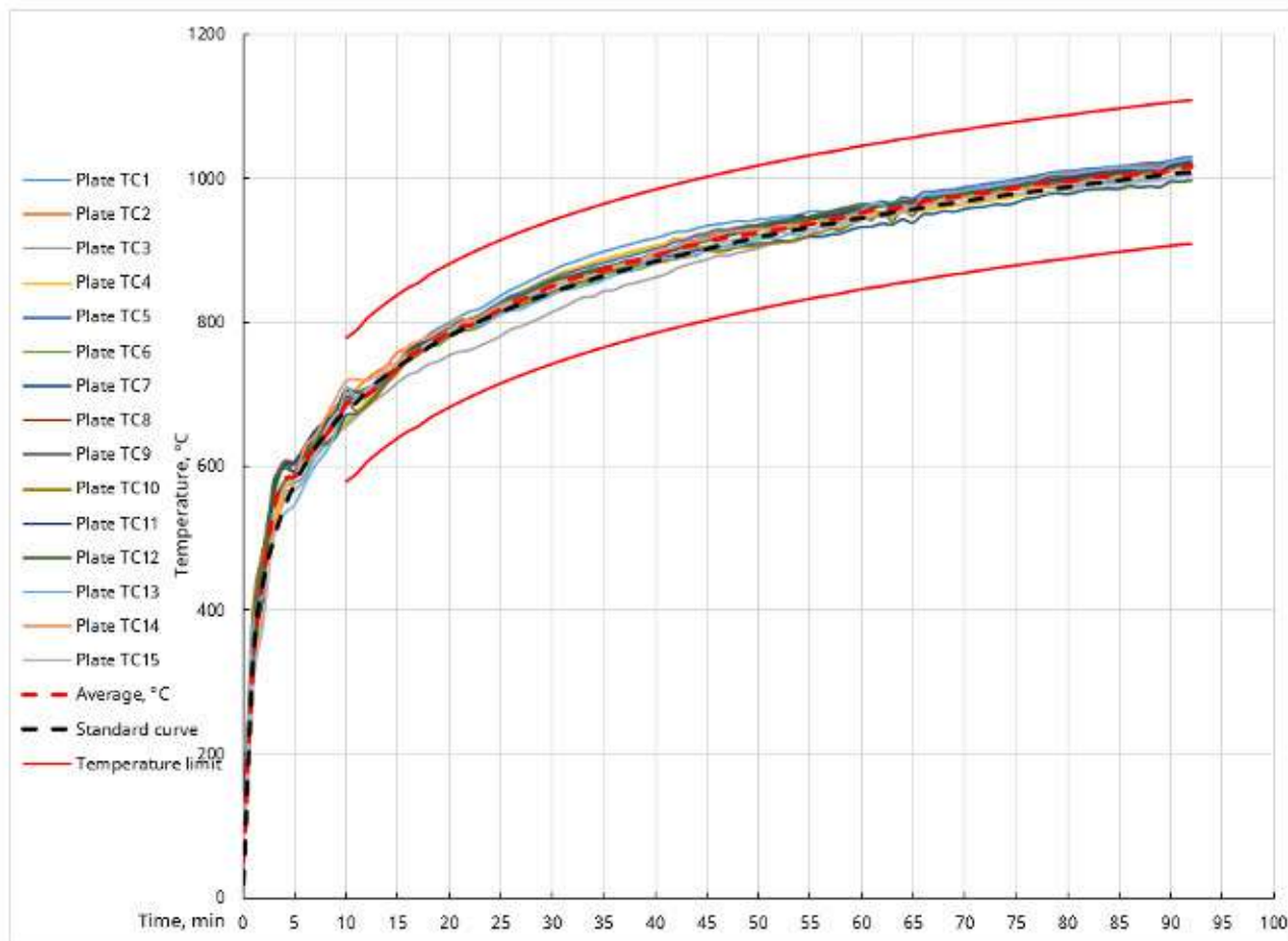
Graph 1. Temperature in the furnace during the test
