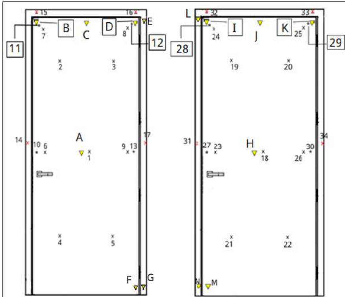
Figure 5. Scheme of the temperature and deflection measuring points on the unexposed side of the door set.
