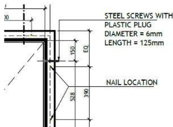
Figure 2. door frame and architrave fixing.
