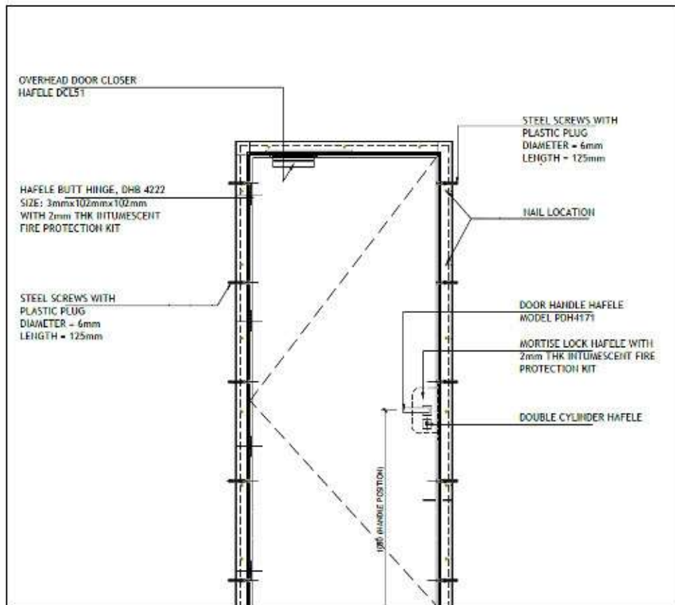
Figure 1. Specimen layout
